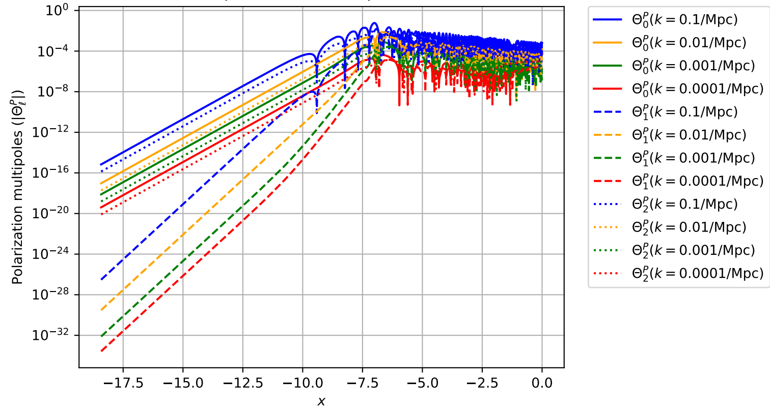
Evolution of polarization multipoles over time (x)
